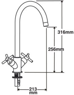
Monobloc High Spout Sink Mixer
